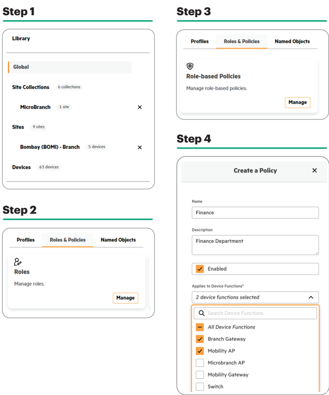
Figure 5. Hierarchical configuration based on business intent
