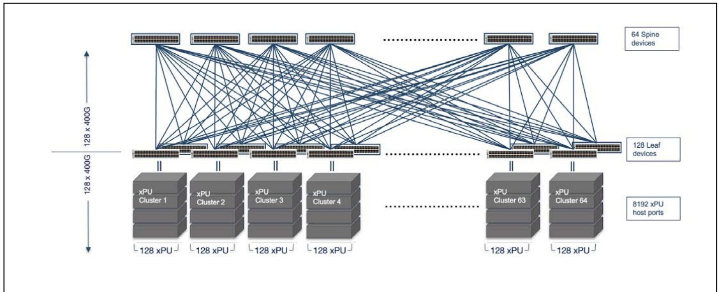
A 2-tier network design using 7060X6 for a 8192 port xPU cluster
